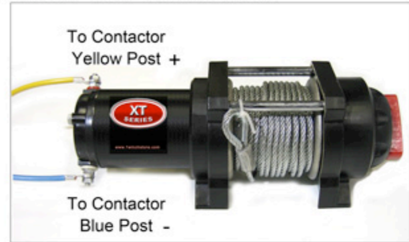
Figure 4 Winch Wiring Diagram - with optional corded remote
