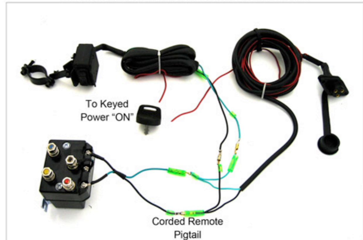
Figure 4 Winch Wiring Diagram - with optional corded remote
